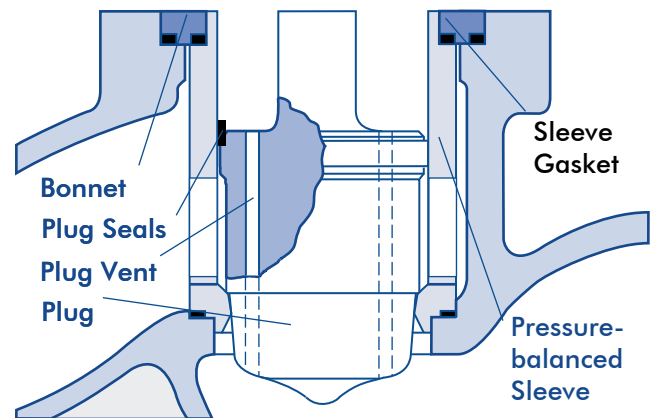
Figure 16: Pressure-balanced Trim
