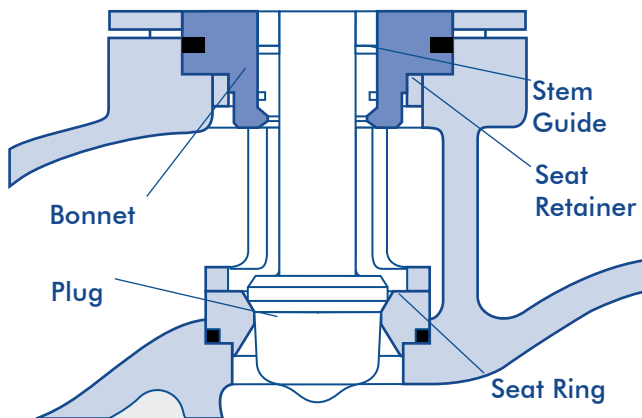
Figure 15: Standard Trim
