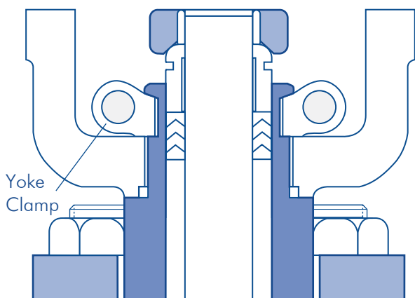
Figure 10: Yoke Clamp
