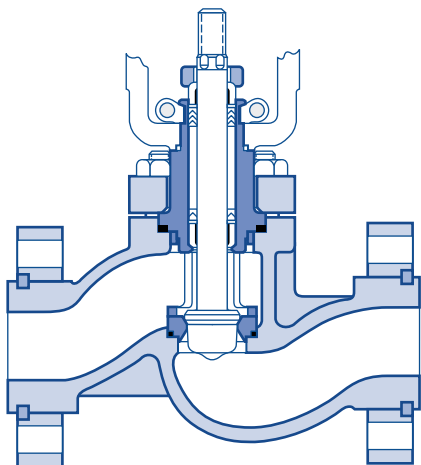
Figure 3: Globe-style body configuration
