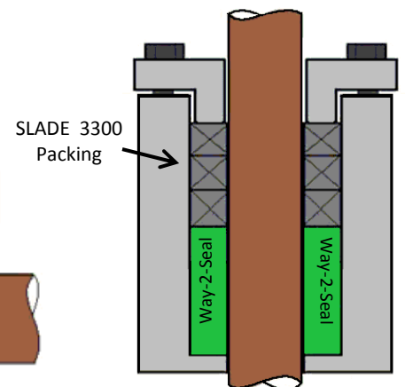
VALVE ARRANGEMENT
