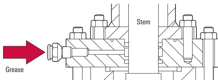
Bonnet-stem seal arrangement showing provision for lubricant or sealant injection.
