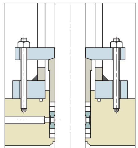
OS&Y bonnet and back seat.
