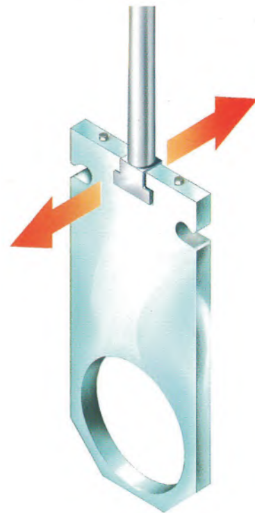
Floating gate-stem connection.
